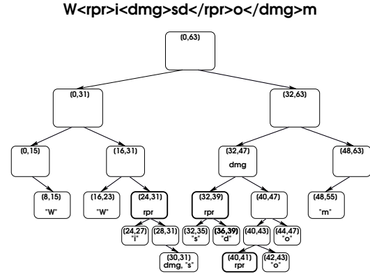
Fig. 5. Modified segment tree
